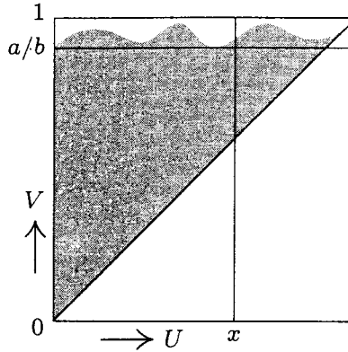
Fig. 11. Region of “acceptance” in Algorithm L.
